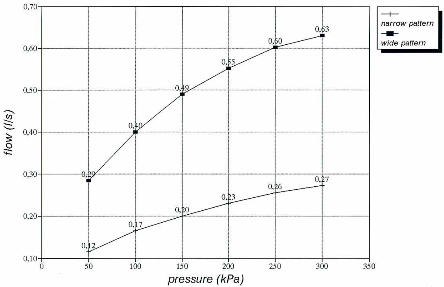
Flow at different pressure conditions ORAS; "SENSIVA" hand shower
